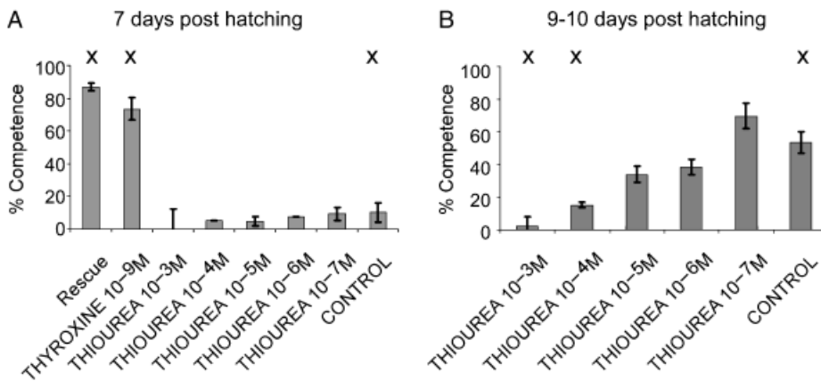
Fig. 1. Thyroxine accelerates development to metamorphosis (A), whereas thiourea leads to an inhibition of metamorphosis in a dose-responsive manner (B). Larvae of Clypeaster rosaceus were induced to metamorphic competence using 80 mM excess KCl on December 11 and December 13/14. (A) While the majority of larvae from the Thyroxine and the Rescue treatment underwent the metamorphic transition upon induction with KCl (i.e., were competent; see text for definition) on 7 days postfertilization, larvae from the Inhibitor treatments and the Control did not reach the threshold of 30% competence (see our definition in text). (B) Two to three days
