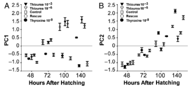
Fig. 2. Thyroxine leads to increased growth of juvenile structures and a decreased growth of larval structures, whereas thiourea reverses this effect in larvae of the sea biscuit Clypeaster rosaceus . We plotted first and second principal component (PC) as a function of time and treatment. PC were derived from eight morphological characters measured on planktonic larvae of C. rosaceus (see Tables 2 and 3) for 48, 72, 100, and 140 h postfertilization. We view PC1 as representative for larval characters, whereas PC2 is representative for the juvenile rudiment (see Table 3). Larvae were exposed to the experimental treatments indicated in the figure legend: Thyroxine ( 10^{-9} M thyroxine); Thiourea 10^{-3} M ( 10^{-3} M thiourea); Thiourea 10^{-5} M ( 10^{-5} M thiourea); and Rescue ( 10^{-9} M thyroxine + 10^{-3} M thiourea). Compared with the control, thyroid hormone synthesis inhibitor has a positive effect on the growth of larval structures (PC1), whereas thyroxine and the rescue treatment led to a negative effect on growth of larval structures (PC1), relative to the control. These effects are reversed for juvenile structures (PC2) and are statistically significant (for details, see text). These results suggest that thyroxine acts as an endogenous signal for the phenotypic plasticity of larval and juvenile structures in C. rosaceus .
