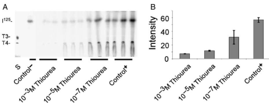
Fig. 4. Larvae of Clypeaster rosaceus incorporate I^{125} and synthesize thyroxine with it. (A) Thin layer chromatography (TLC) plate showing T4 (thyroxine) band but not T3 (3,3',5-L-triiodothyronine). (B) Measurement of intensity of putative T4 bands for all treatments and the control. Both iodine incorporation (data not shown) and thyroxine synthesis are inhibited by thiourea (A, B). Larvae were exposed to I^{125} for 18 h in the presence ( 10^{-3} M Thiourea, 10^{-5} M Thiourea, 10^{-7} M Thiourea) and absence (Control+)
