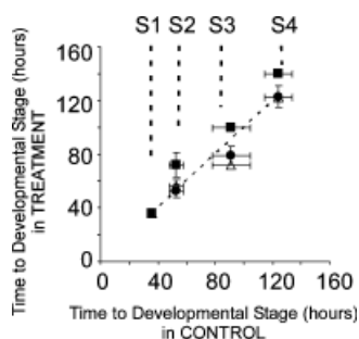
Fig. 3. Thyroxine treatment does not lead to a consistent heterochronic shift in development for Clypeaster rosaceus facultative feeding larvae. The graph represents heterochrony plot for the following treatments: ●, Thyroxine ( 10^{-9} M thyroxine); ■, Thiourea 10^{-3} M ( 10^{-3} M thiourea) Δ, Rescue ( 10^{-9} M thyroxine + 10^{-3} M thiourea). Each point in a heterochrony plot represents the mean value of time to a particular developmental stage (for developmental stages S1–S4, see text and Heyland and Hodin 2004). The y-axis information is the timing of larvae to a developmental stage from a given treatment. The x-axis represents the corresponding timing of control (i.e., unfed) larvae to reach the same developmental stage. Note that the error bars are SE of the mean based on four independent replicates. The dotted black line represents the standard and represents the developmental timing of control versus control. All points that lie below this black line represent accelerated development. All points above the black line represent decelerated development. No significant difference between treatments and the control were detected ( P < 0.05 ).
