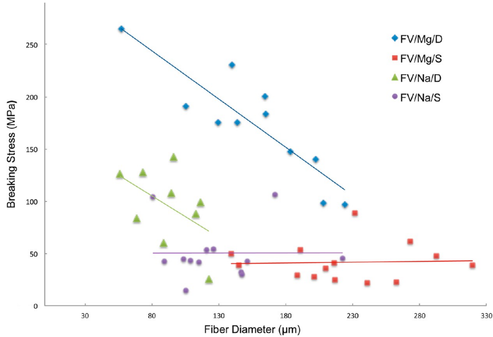
Figure 6. Fiber breaking stress plotted against diameter for four of the FV treatments. Strength was inversely proportional to diameter within FV/Na/D and FV/Mg/D fibers but had no effect on FV/Na/S and FV/Mg/S fibers. These data demonstrate that the superior mechanics of FV/Mg/D fibers are not driven by effects of Mg^{2+} on fiber diameter.
