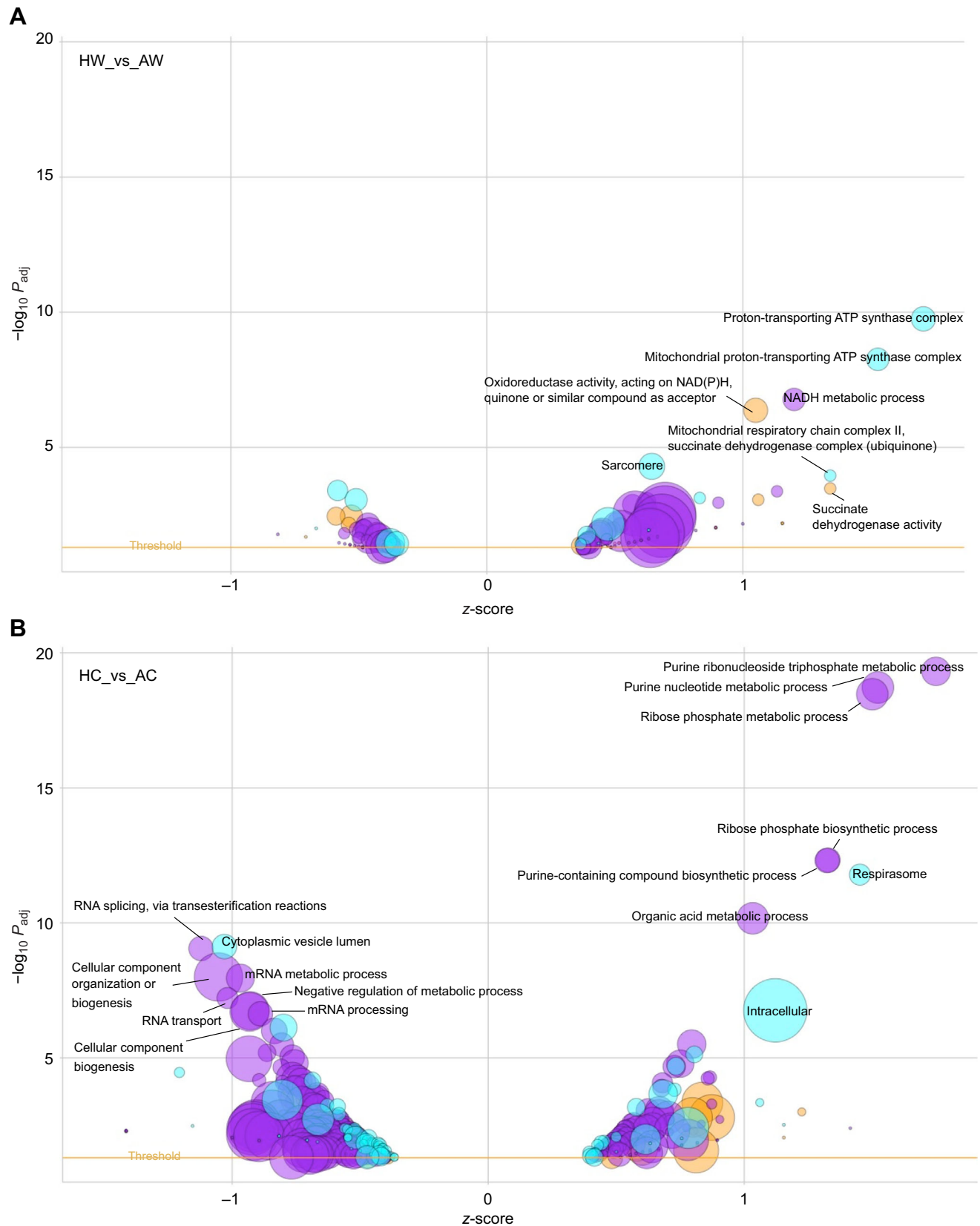
Fig. 6. Enriched GO terms for the stage \times temperature interaction that are unique from a main effect of life stage. Data for (A) warm-acclimated hatchlings relative to adults (HW_vs_AW) and (B) cold-acclimated hatchlings relative to adults (HC_vs_AC) are plotted as the inverse log of the adjusted P -value versus z -score. Positive and negative z -scores indicate GO term enrichment for proteins that increase or decrease in abundance from hatchling to adult, respectively. Bubble size corresponds to the number of DA proteins represented in the GO term. Bubble colour corresponds to the primary GO terms biological process (purple), cellular component (blue) and molecular function (orange). A selection of the top up-regulated and down-regulated GO terms is labelled.
